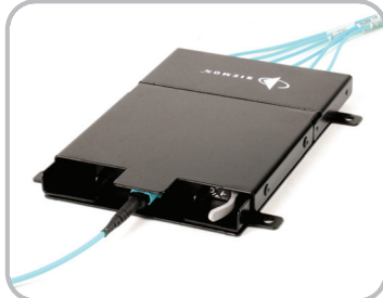
Plug and Play – LightStack MTP to LC module (not included) accepts an MTP trunk cable at the rear for fast deployment and pathway space savings.
